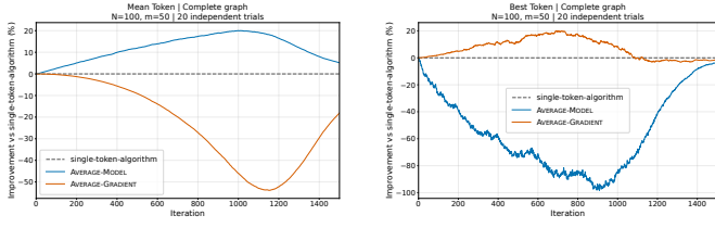
(a) Mean-token loss improvement (b) Best-token loss improvement
