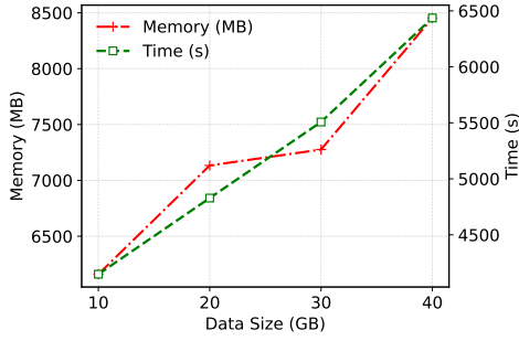
Fig. 6. Scalability analysis in terms of memory consumption and training time.
