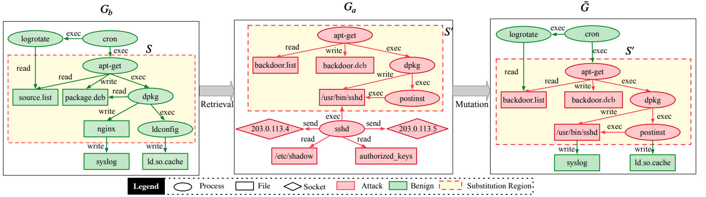
Fig. 3. Structural mutation example. The subgraph S in benign graph G_b is replaced by the aligned attack subgraph S' from G_a , producing the mutated graph \tilde{G} where the attack structure (red) is embedded within benign context (green).
