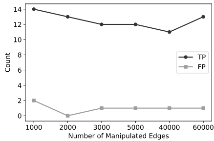
Fig. 10. Detection results under mimicry attacks.
