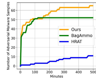
Fig. 5. Runtime efficiency comparison with other state-of-the-art methods.
