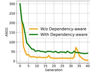
Fig. 4. Impact of dependency-aware strategy.
