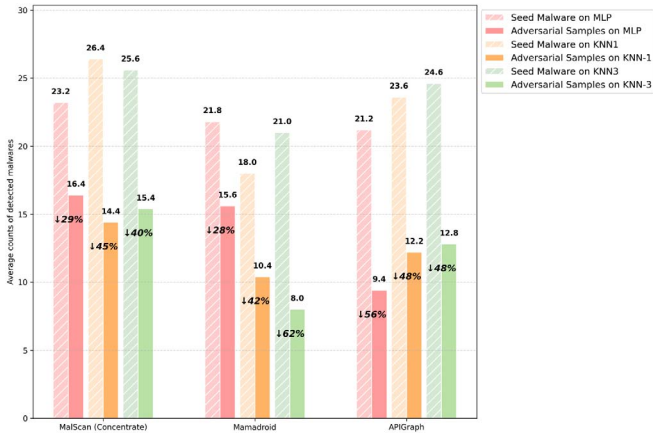
Fig. 6. Detection score difference between malware and corresponding adversarial samples.
