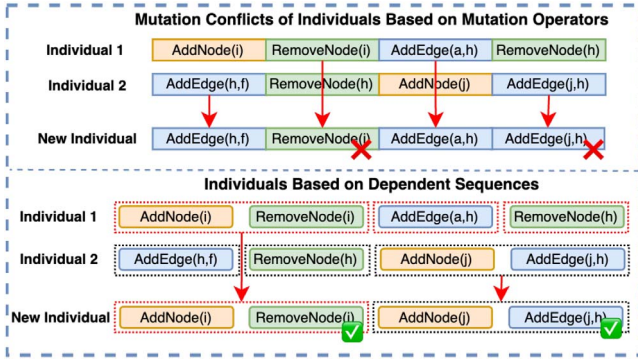
Fig. 2. Crossover with/without dependency strategy.
