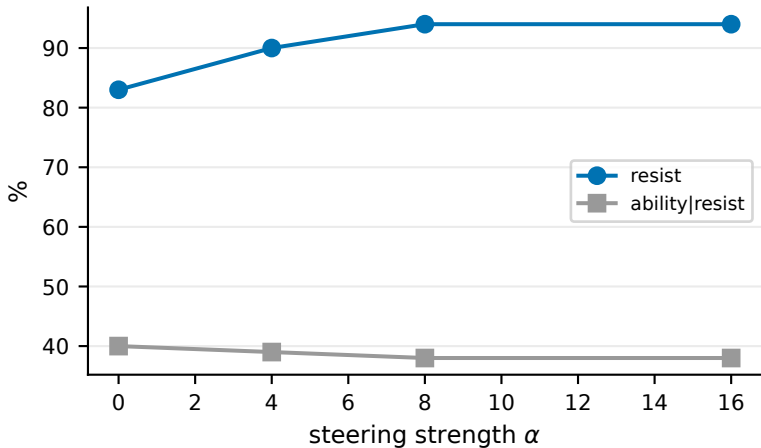
Qwen3-8B: decision moves, computation flat
