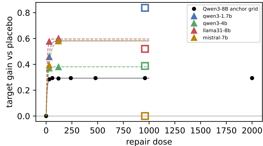
FMT: fitted ( \blacktriangle , low doses) vs held-out prediction ( \square , high dose)
