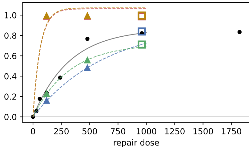
ANS: fitted ( \blacktriangle , low doses) vs held-out prediction ( \square , high dose)
