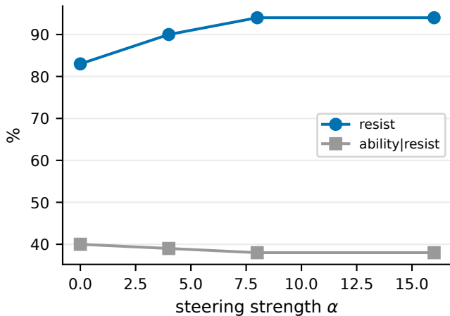
(a) Qwen3-8B: decision moves, computation flat
