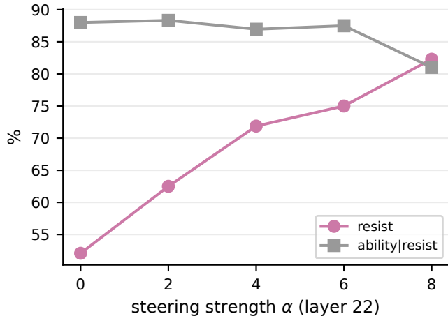
(b) Llama-3.1-8B: the lever transfers
