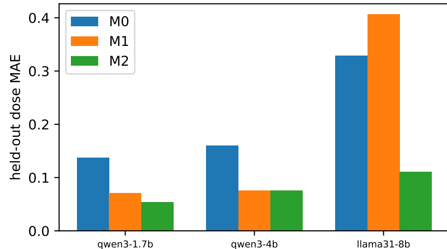
Adaptation level vs held-out error (M2 tau declared optimistic)
