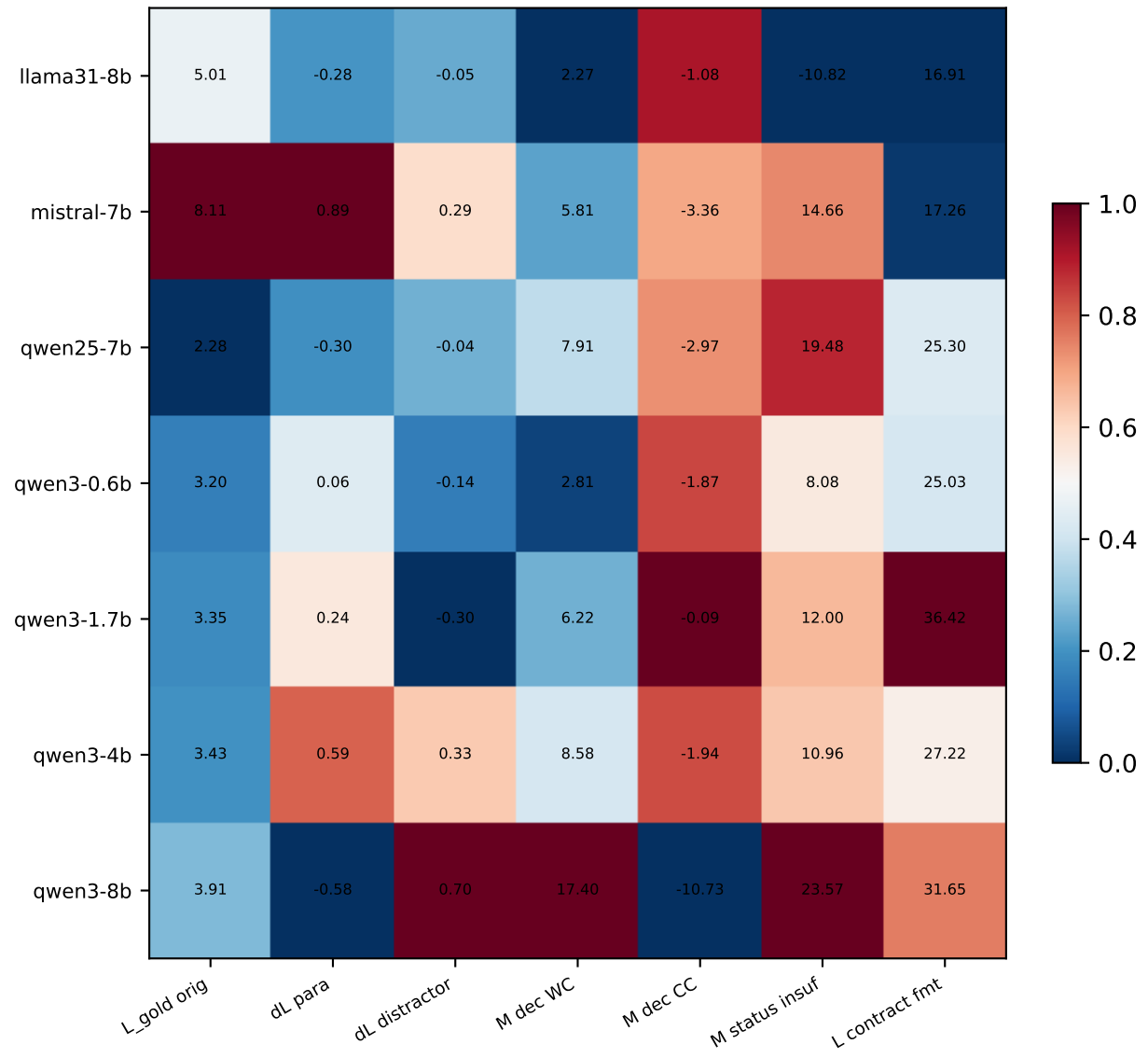
loss / margin (col-normalized; annot = raw)
