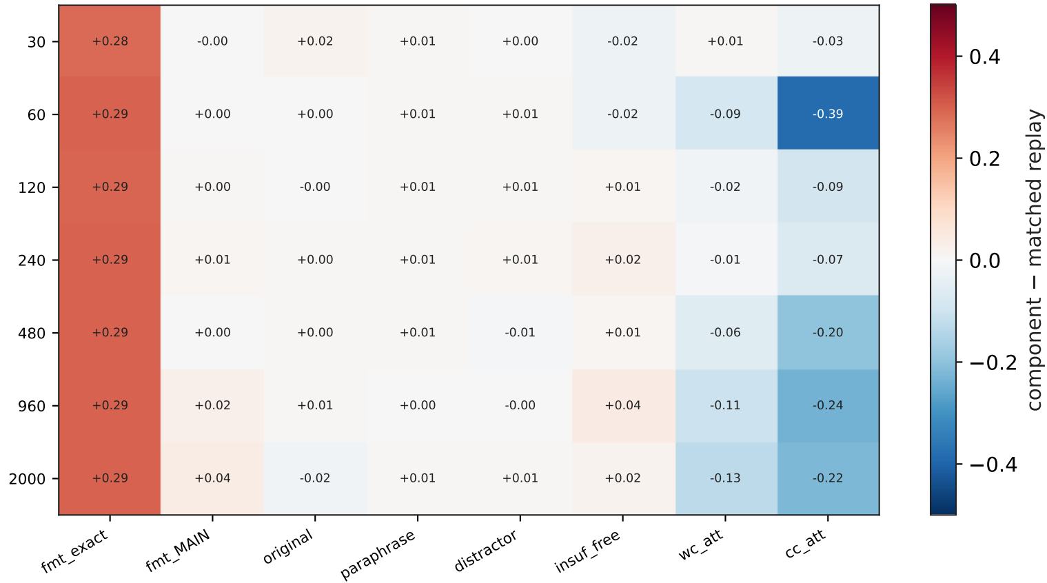
Fig 4 — Format response vector vs matched replay [eval-500; n: core=529 fam; insufficient/STATUS=249; NL=100; paraphrase=50 (frozen subsets)]
