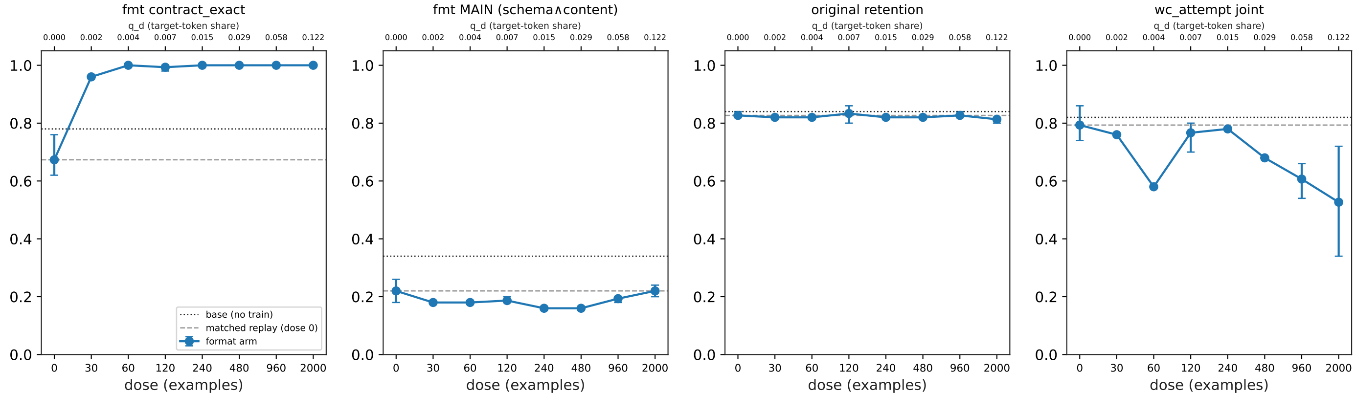
Fig 3 — Format formal dose response (2,000-example carrier; packed; 30 updates all arms; budget PASS)
