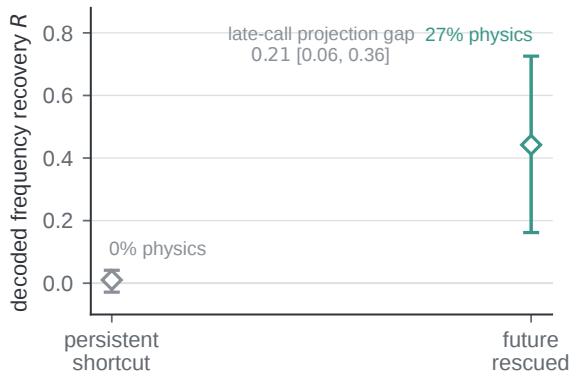
b More target write, more decoded rescue
