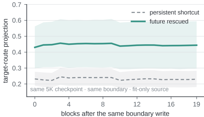
a Future-rescued errors realize more of the route
