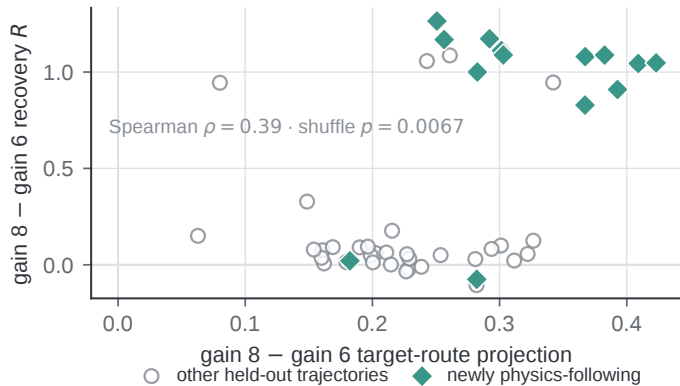
a Route-aligned write predicts decoded rescue
