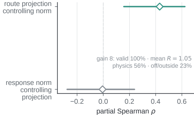
b Route signal survives norm control
