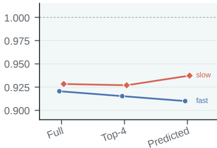
a Predicted write approaches matched Top-4
