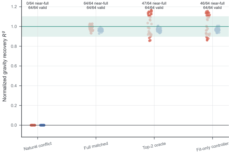
Free fall: donor-free held-out recovery at rank 2 (representative eval_50281_low)
