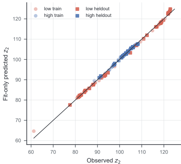
Causal coordinate z_2
