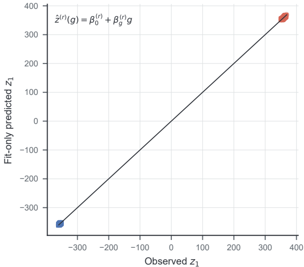
Causal coordinate z_1
