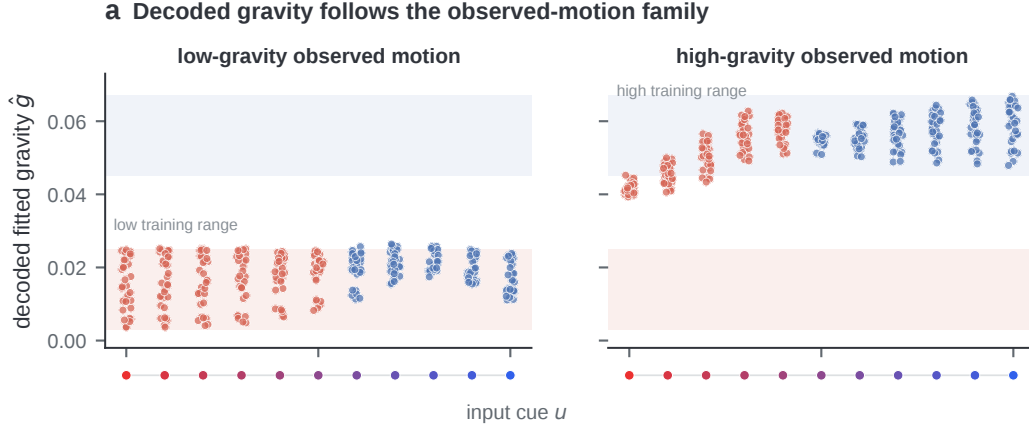
Figure 19: Decoded Free Fall gravity follows the observed-motion family. Holding low- or high-gravity observed motion fixed in the 32-frame regime, we sweep 11 appearance cues and fit \hat{g} from all 704 decoded futures. Point color is measured future appearance; pale bands show the two training-supported gravity ranges.
