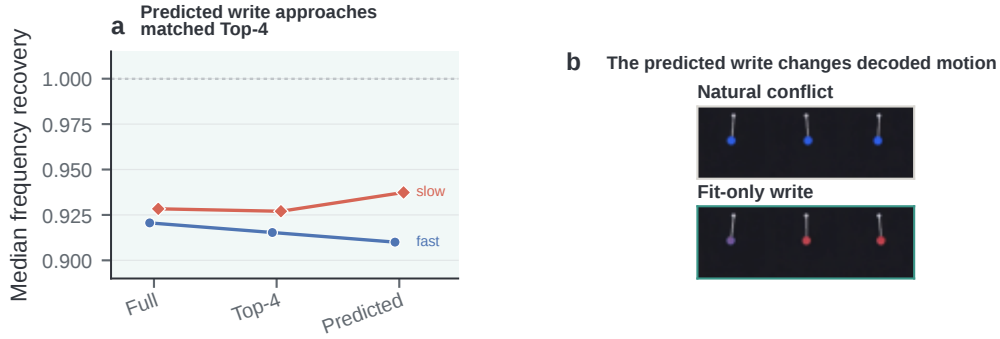
Figure 17: A donor-free top-four Pendulum controller approaches the Top-4 reference. a , Fast- and slow-target medians among evaluator-valid receivers compare Full, Top-4, and predicted writes in the same coordinate space. b , Real decoded strips show the same held-out receiver before and after the fit-only write. All-cohort validity and near-full counts are reported in the accompanying text.
