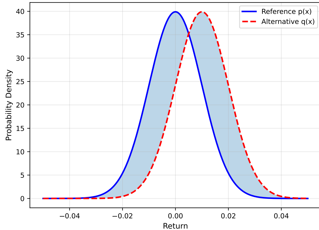
(c) Shifted Distribution KL Divergence = 0.1250
