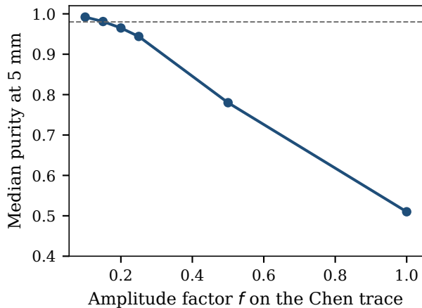
L = 5 mm, scaled Chen trace
