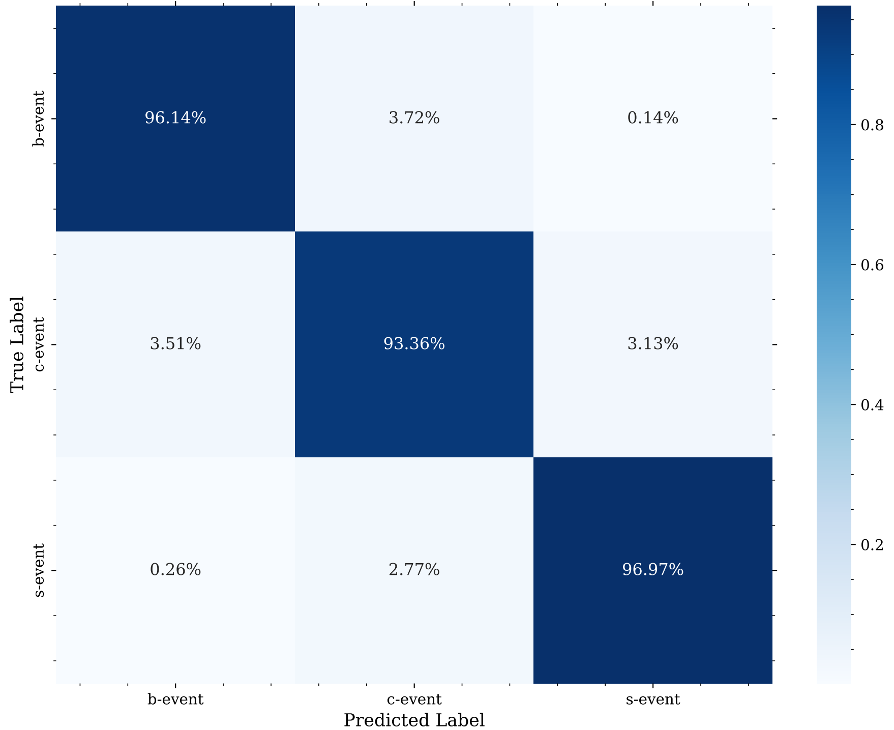
Normalised Confusion Matrix
