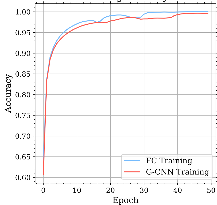
Training Accuracy
