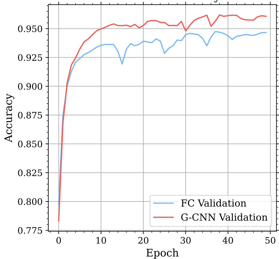
Validation Accuracy
