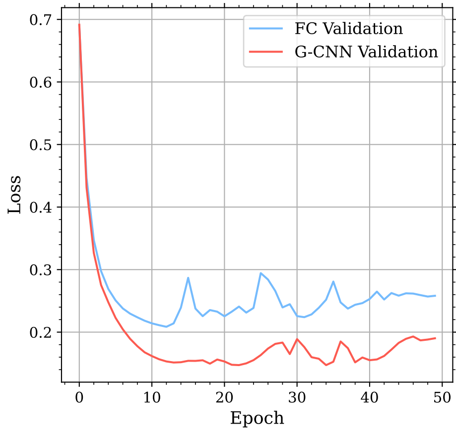
Validation Loss
