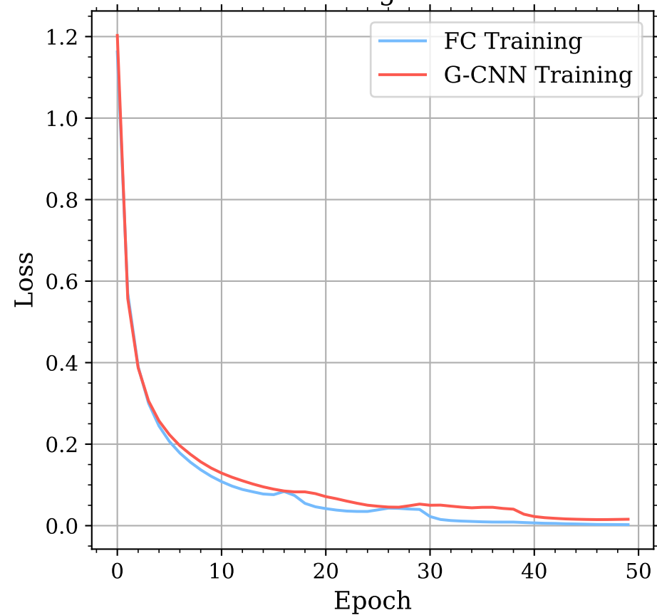
Training Loss
