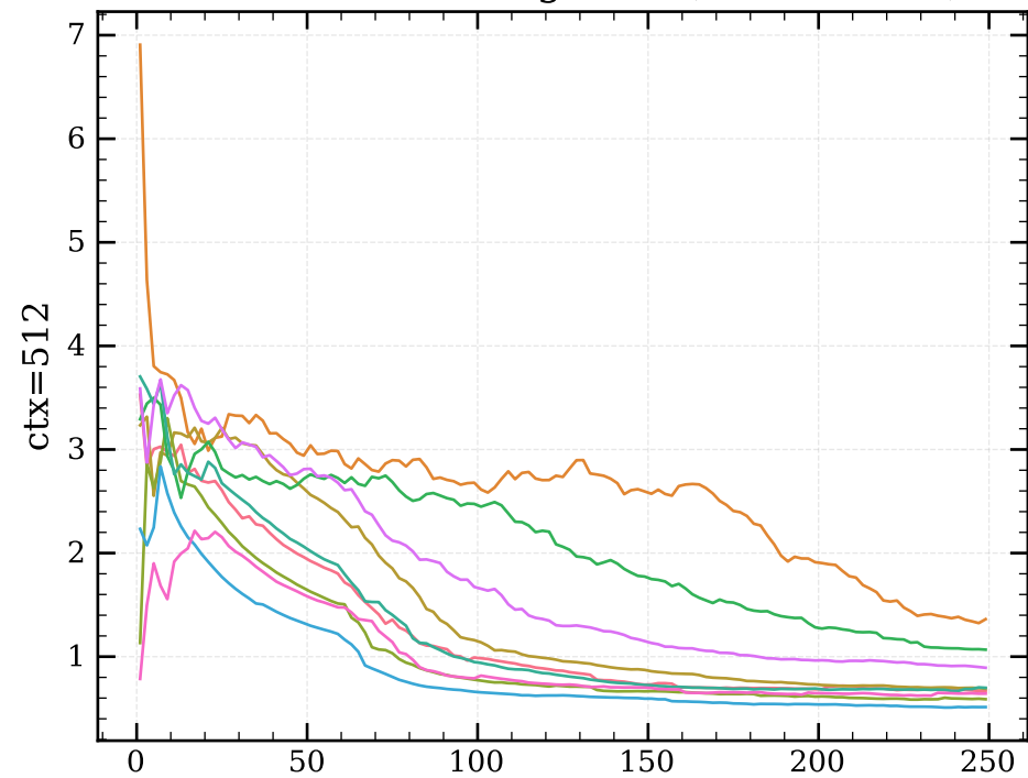
Smoothed Training Loss (window=30)
