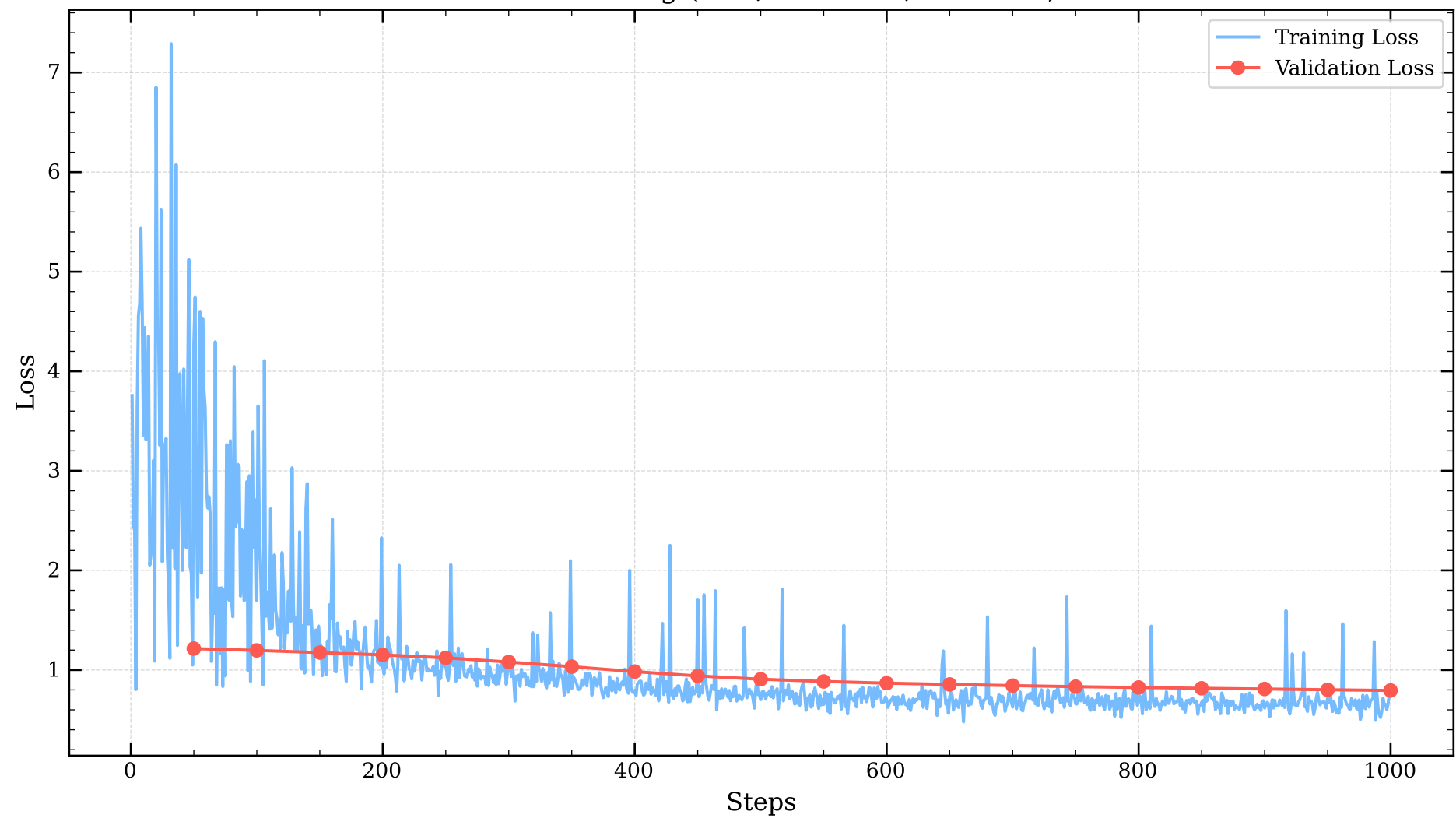
LoRA Training (r=4, lr=1e-05, ctx=512)
