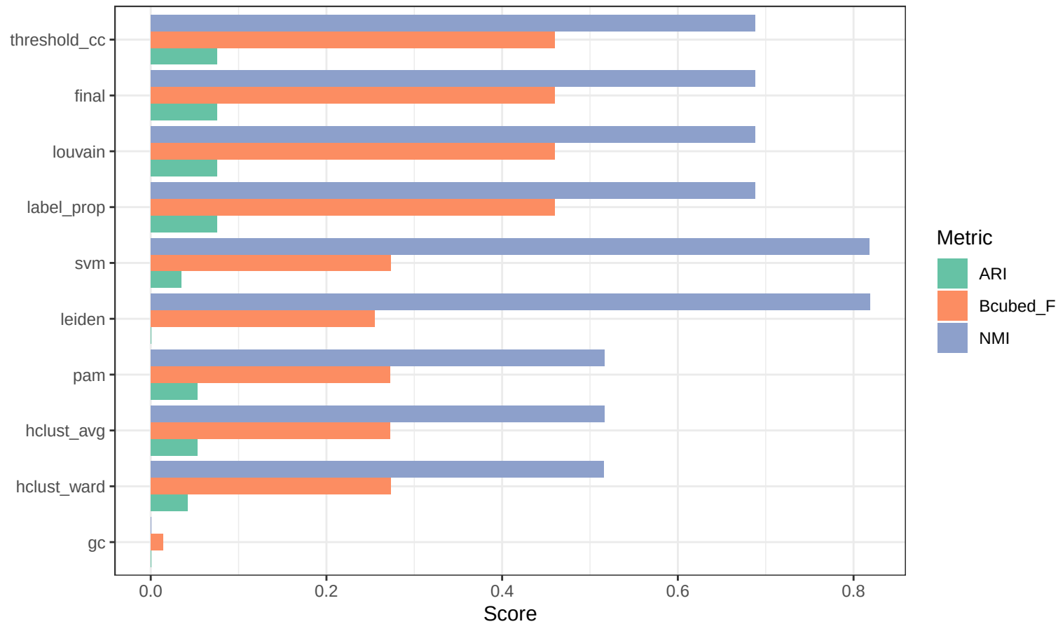
Affiliation — Method Comparison
