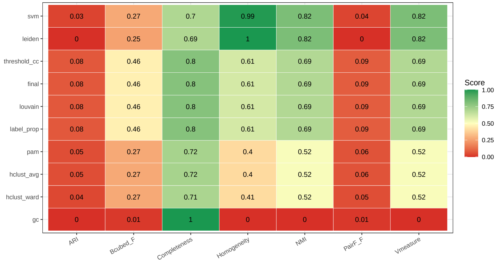
Affiliation — Performance Heatmap
