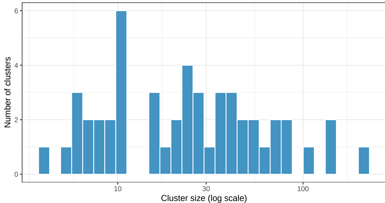
CORA — Cluster Size Distribution (final)
