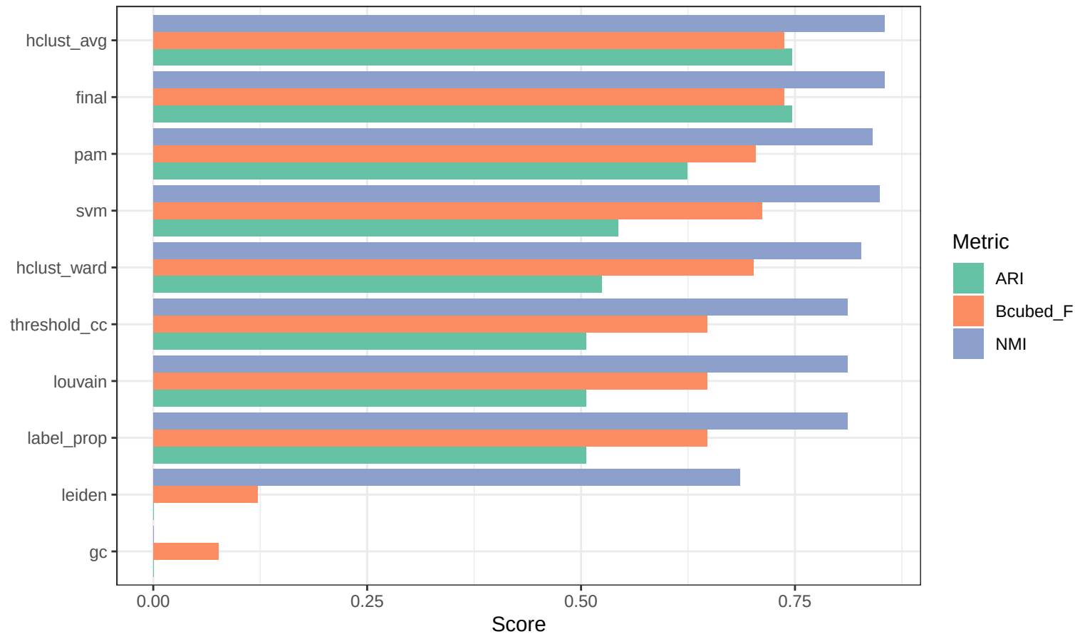
CORA — Method Comparison
