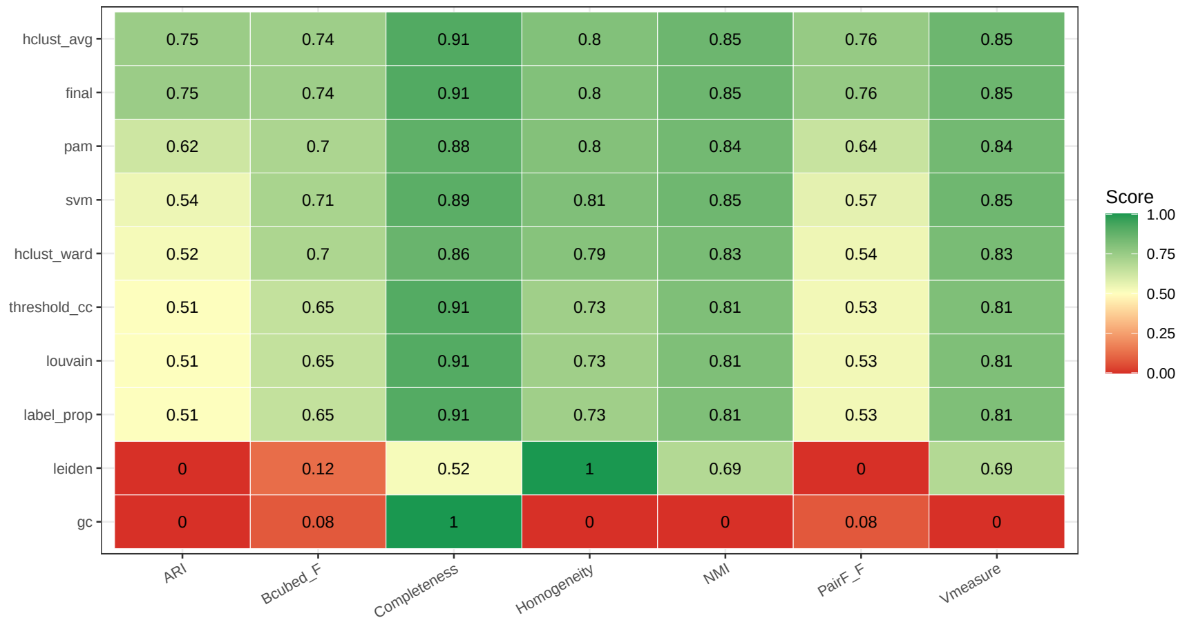
CORA — Performance Heatmap
