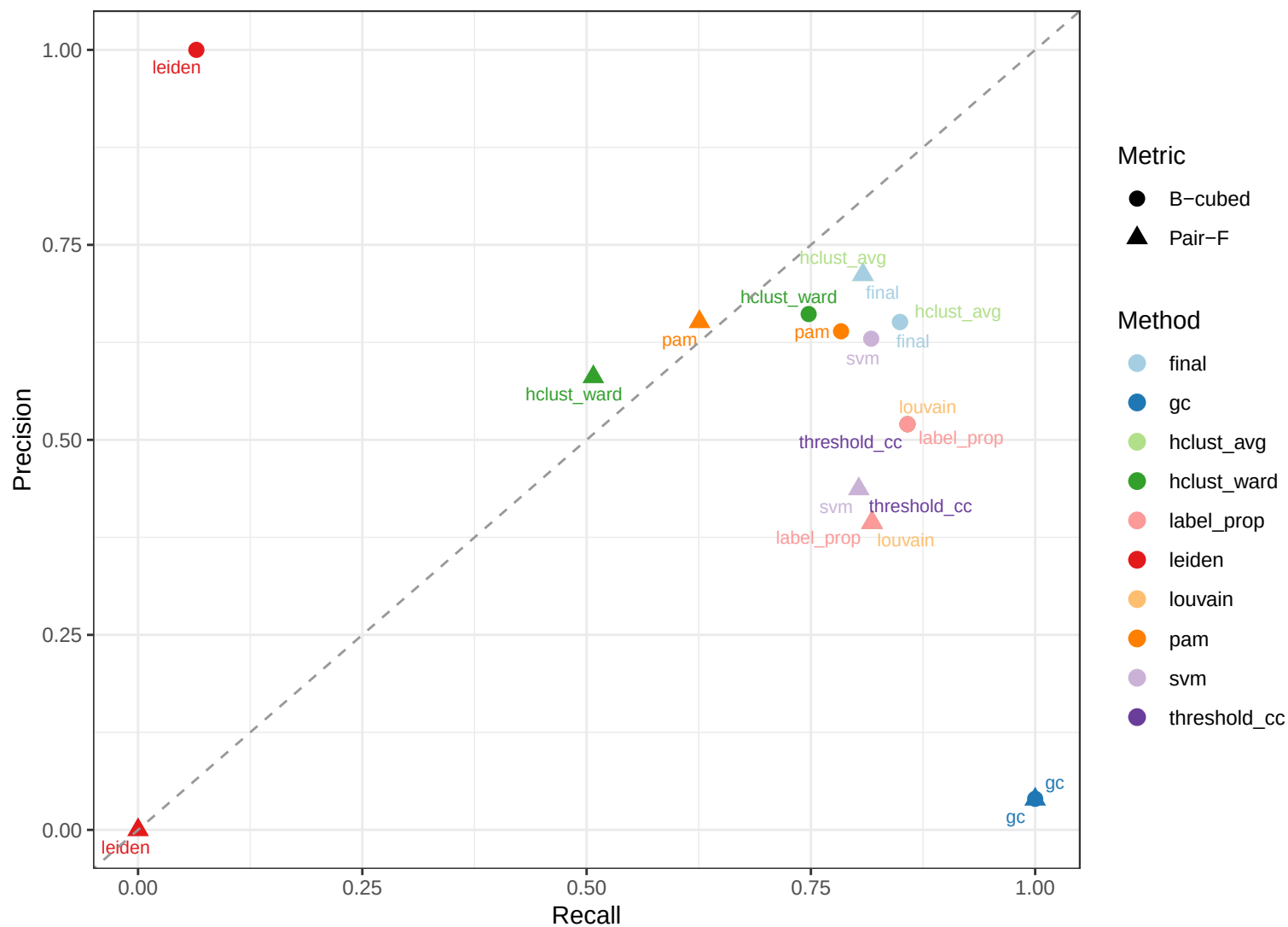
CORA — Precision vs Recall
