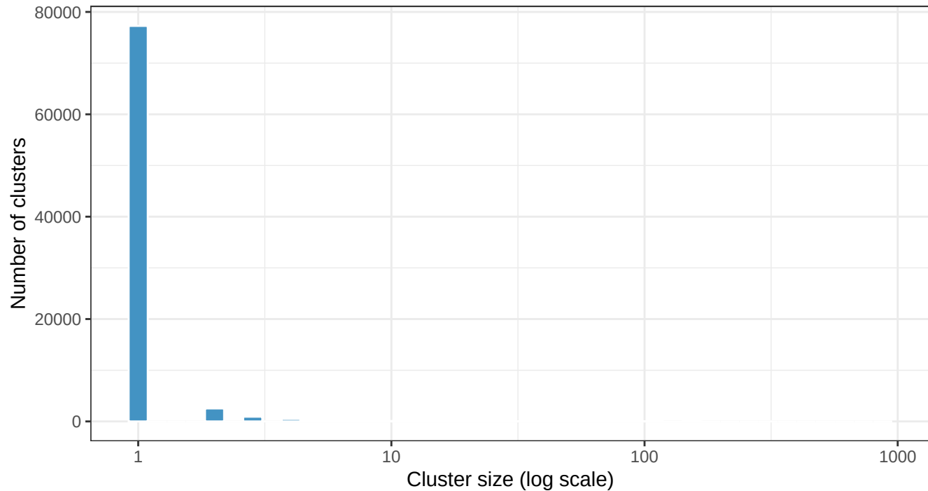
NCVR10 — Cluster Size Distribution (final)
