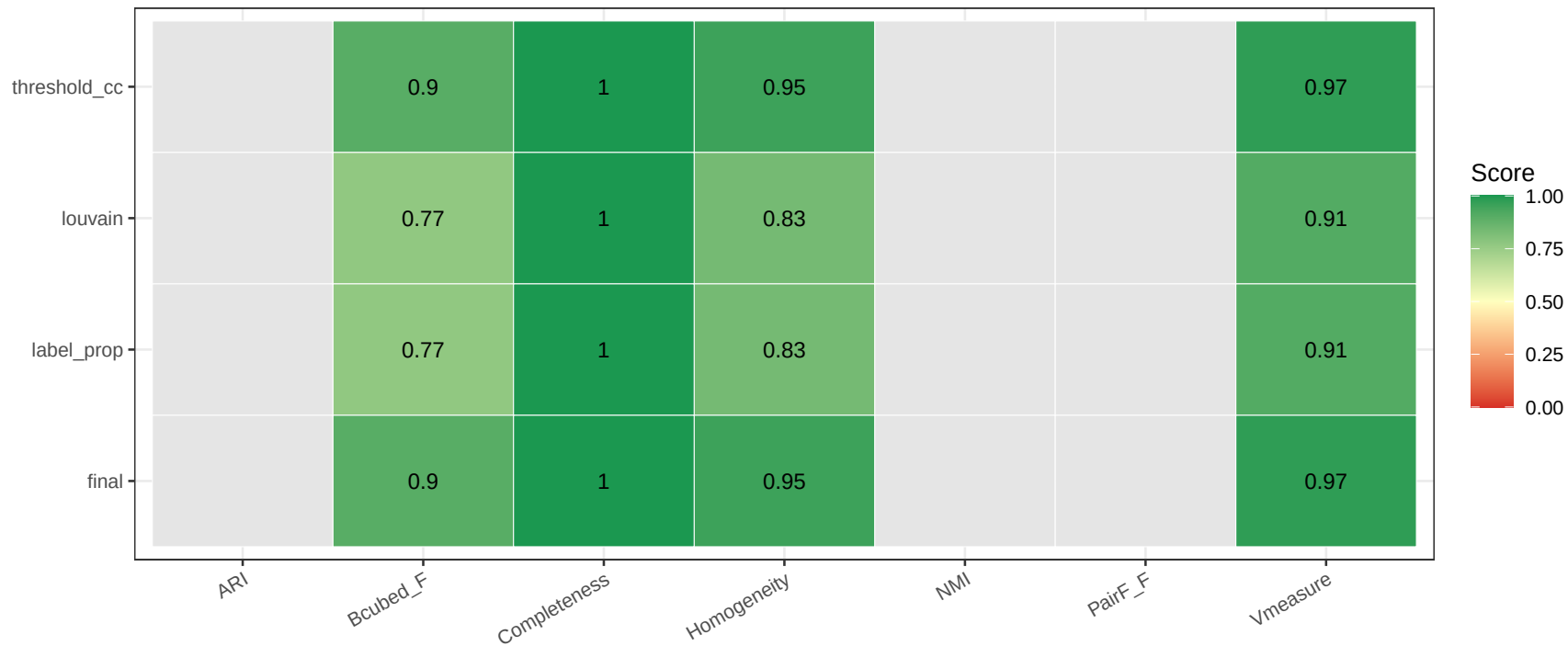
NCVR10 — Performance Heatmap
