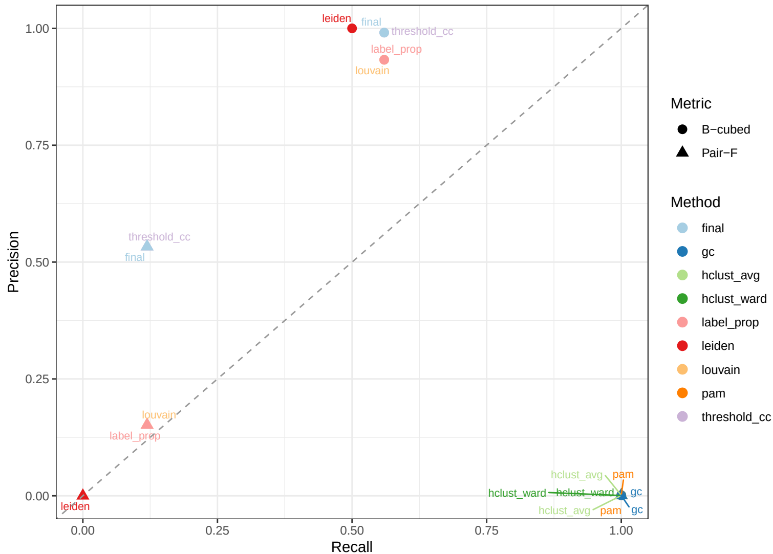
NCVR5 Large — Precision vs Recall
