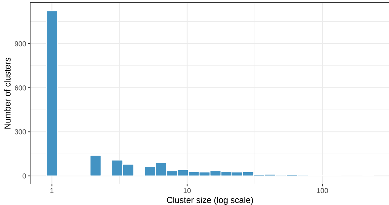
NCVR5 Small — Cluster Size Distribution
