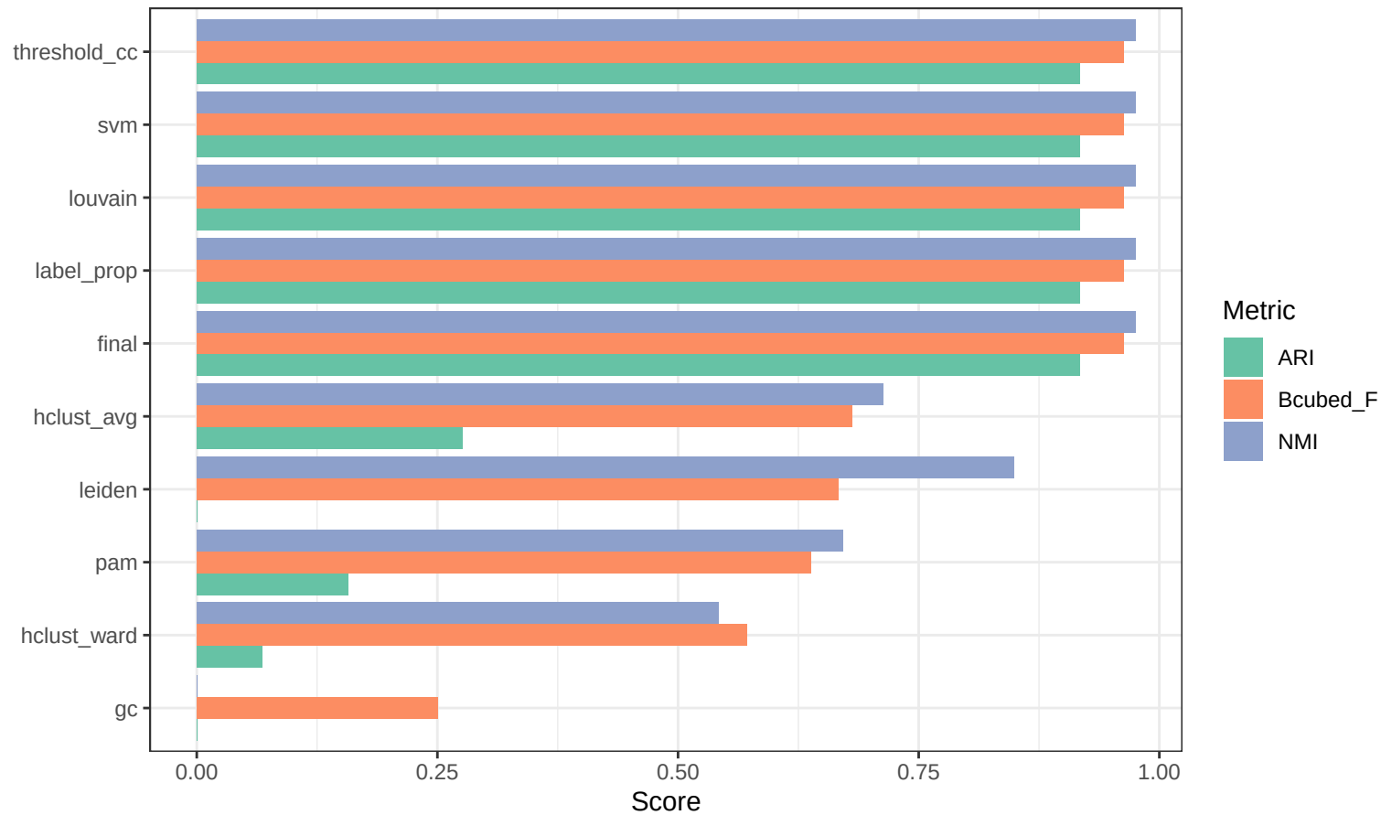
NCVR5 Small (5K/party) — Method Comparison
