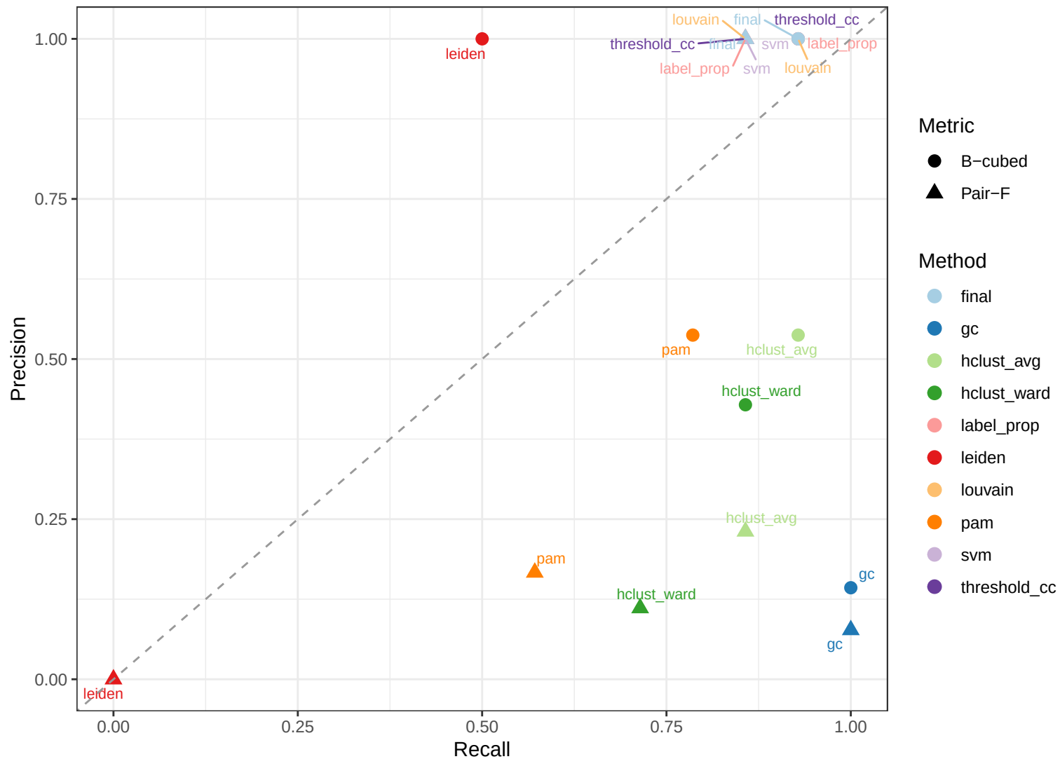
NCVR5 Small — Precision vs Recall
