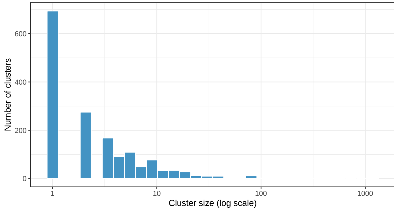
Syn10k — Cluster Size Distribution (final)
