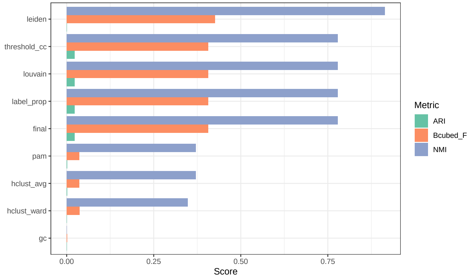
Syn10k — Method Comparison
