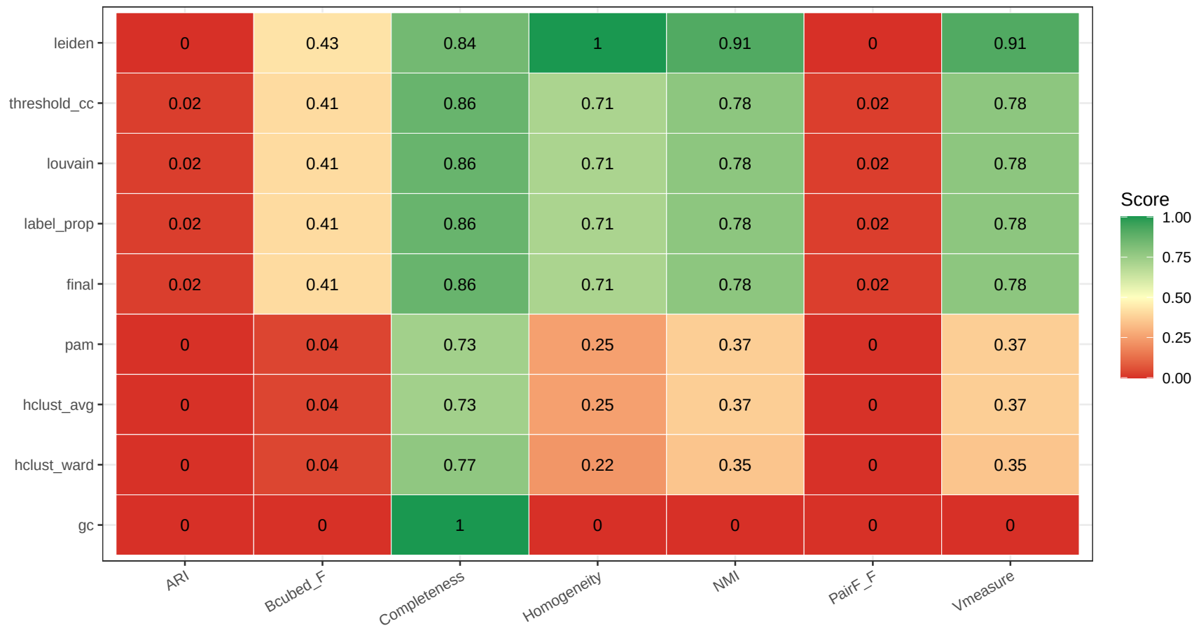
Syn10k — Performance Heatmap
