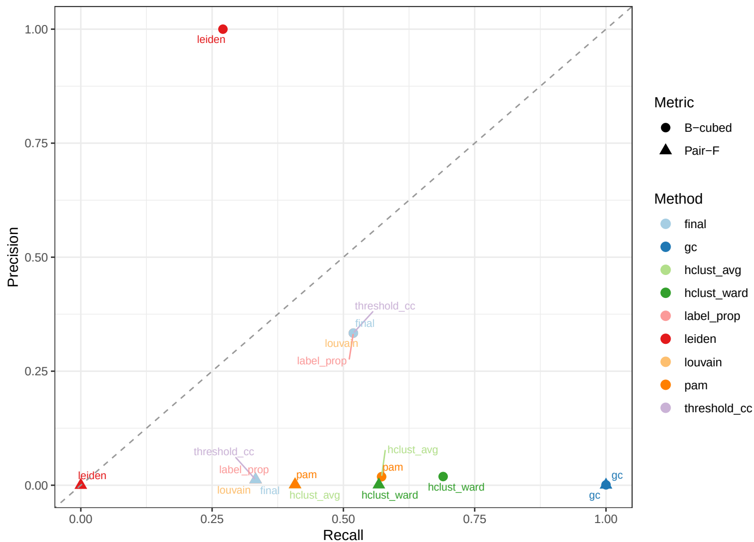
Syn10k — Precision vs Recall
