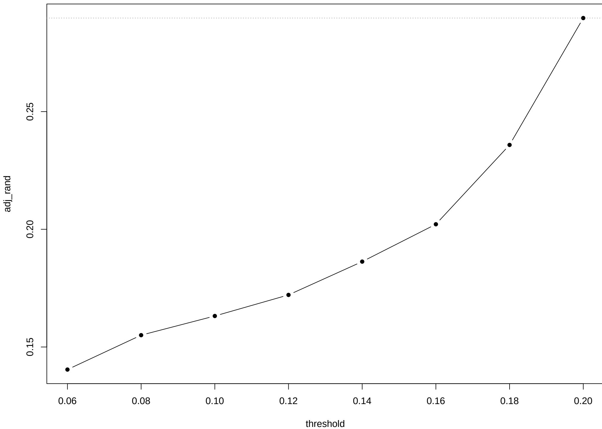
GC tuning — adj_rand vs threshold
