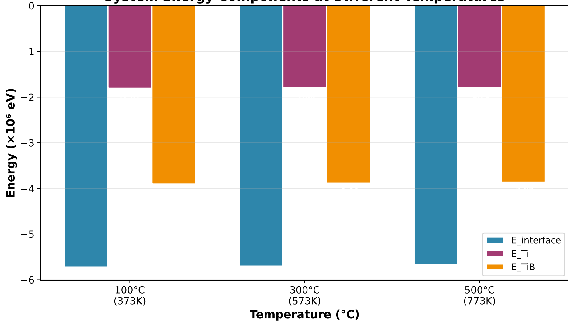
System Energy Components at Different Temperatures
