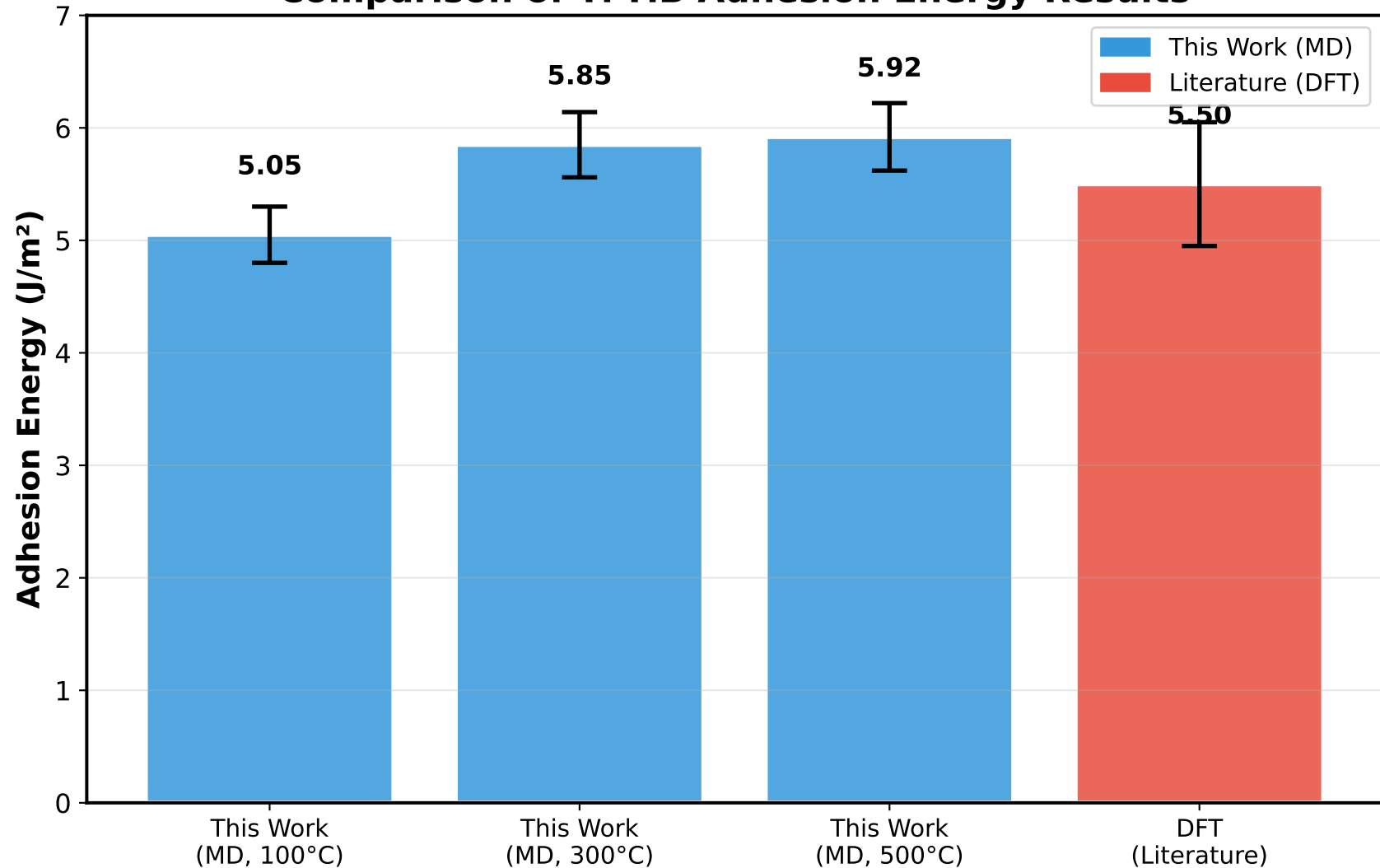
Comparison of Ti-TiB Adhesion Energy Results
