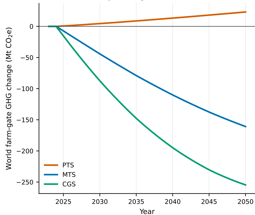
a SSP2 annual pathway
