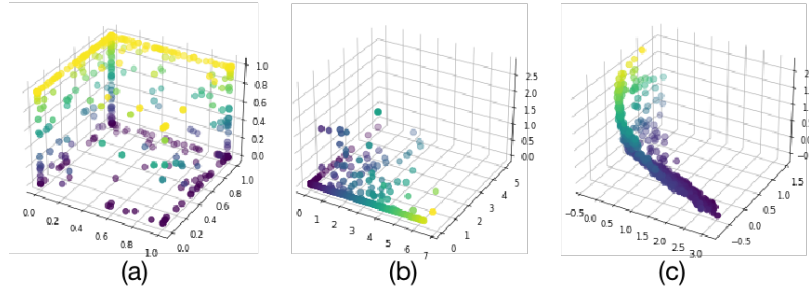
Figure 6: Marginal distributions of a random digit in the MNIST. (a) Raw pixel space. (b) Encoded feature space learned by a typical AE. (c) Encoded feature space learned by ours. The manifold can be well preserved.
