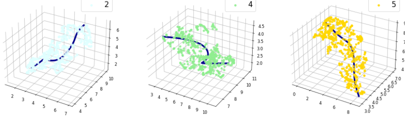
Figure 3: Principal curves of MNIST digits. Blue lines denote learned principal curves, which summarize the trajectory of each digit manifold in the visualized feature space.
