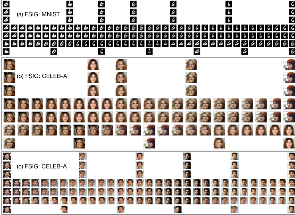
Figure 11: Visualization of generated samples on MNIST and CELEB-A in the FSIG setting. Row 1: the original seven samples. Row 2: AE reconstructions of the seven samples. Row 3: reconstructions from projected points on the intrinsic manifold. Row 4: linear interpolation in the predicted order. Row 5: spline interpolation in the predicted order. Row 6: linear interpolation in a random order. Row 7: real samples corresponding to the random samples in Row 6.
