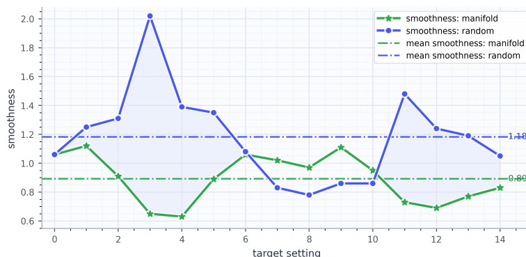
Figure 10: Smoothness of generated samples on CELEB-A. Dashed horizontal lines show the mean smoothness for each ordering strategy. The predicted order along the intrinsic manifold yields smoother transitions than a random order.
