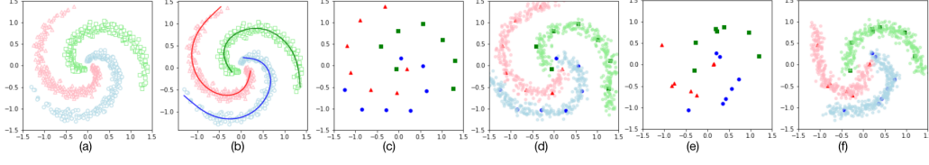
Figure 5: Illustration of our proposed method on generating data along the intrinsic manifold (Best viewed in color). Different colors indicate different classes. (a) Ground-truth dataset. (b) Manifold in each class. (c) Provided 7 representative shots in each class. (d) Reconstructed manifold from (c) and the corresponding generated samples along the manifold. (e) Randomly chosen 7 shots and (f) Manifold reconstructed from (e). In contrast to others that either use linear interpolation or Gaussian augmentation, our method is capable of generating samples along the intrinsic manifold.
