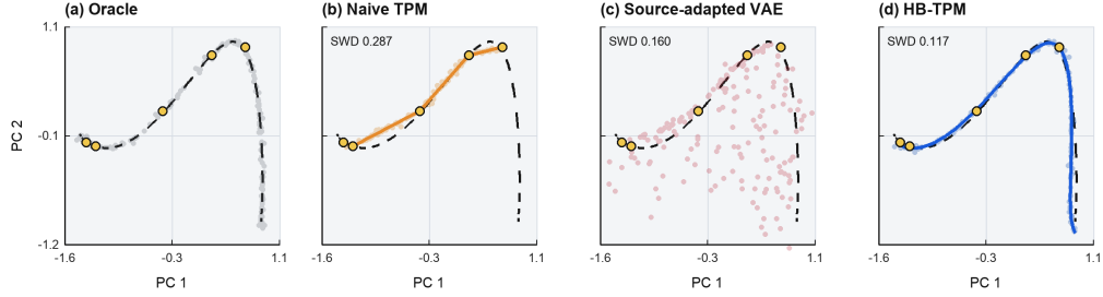
Figure 7: Held-out trajectory recovery for repeat 0 with K = 5 . All panels use the same PCA projection learned from the true eight-dimensional curve and identical axis limits. The black dashed line is the oracle curve, gold markers are the five unordered target shots, colored points are generated or oracle samples, and solid lines are explicit fitted trajectories. Naive TPM connects only the locally covered shots; the source-adapted VAE produces a broad point cloud without a unique explicit path; HB-TPM uses the ordered-source prior to recover the unobserved bend and obtains the lowest SWD. This example is explanatory; statistical conclusions use all 30 held-out tasks.
