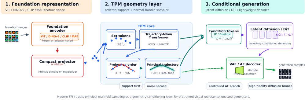
Figure 2: Modern trajectory-aware principal-manifold framework. TPM is inserted as a geometry-conditioning layer between a pretrained visual representation and a generator. A foundation encoder such as ViT, DINOv2, CLIP, or MAE produces semantic tokens, an intrinsic-dimension projector compacts the target representation, and a trajectory-token module recovers projection order and a principal trajectory. The resulting TPM condition tokens constrain either a latent diffusion/DiT branch for high-fidelity synthesis or a lightweight AE/VAE decoder branch used in controlled experiments.
