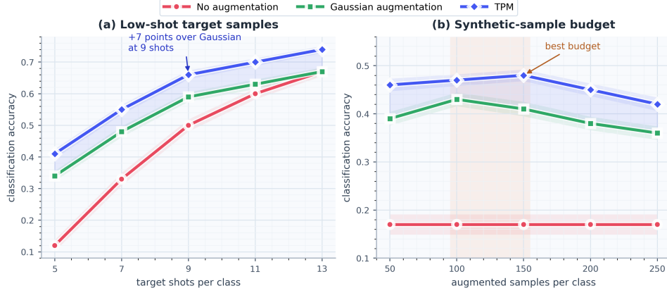
Figure 9: MNIST few-shot classification under different target-shot budgets and synthetic-sample budgets. Shaded bands indicate small run-to-run variation; the no-augmentation curve in the synthetic-budget panel is shown as a fixed reference. TPM gives the largest gain in the low-shot regime and peaks at a moderate augmentation budget.
