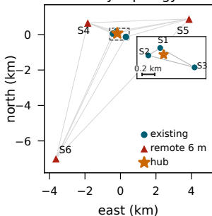
Array topology
