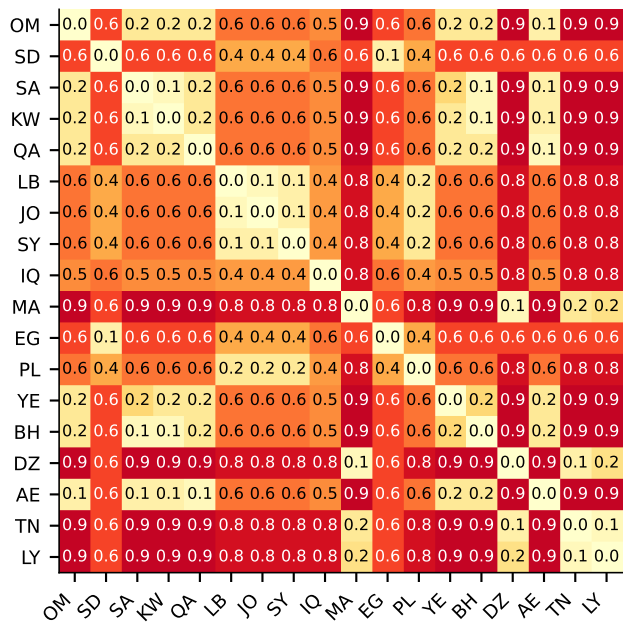
(a) NADI 2024 18-way
