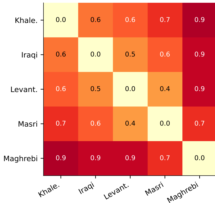
(b) NADI 2024 5-way (coarse)
