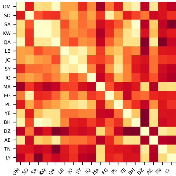
(a) AraBERT feature distance
