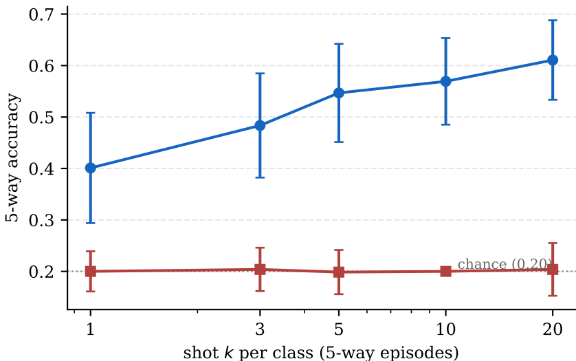
Support size vs. accuracy on NADI 18 (seed 42)
