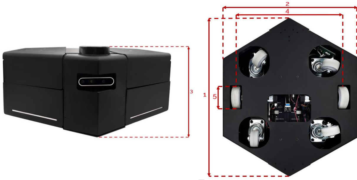
Figure 13. QBot Dimensions
