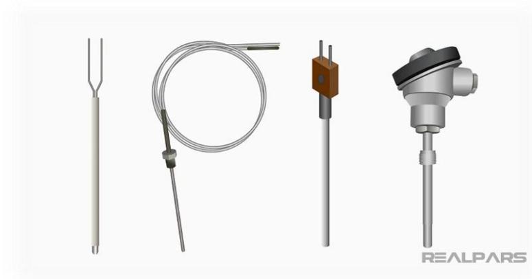
Figure 1: Different forms of thermocouples. Image source: https://www.realpars.com/blog/thermocouple
